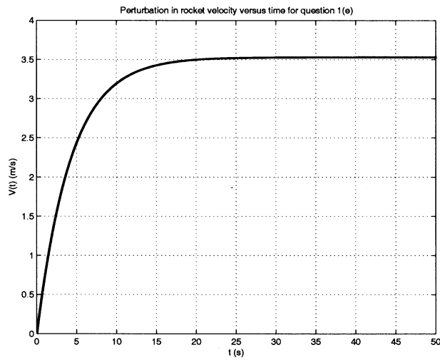
Figure 2: Velocity perturbation response of rocket with step input in thrust perturbation of magnitude 0.1N.
