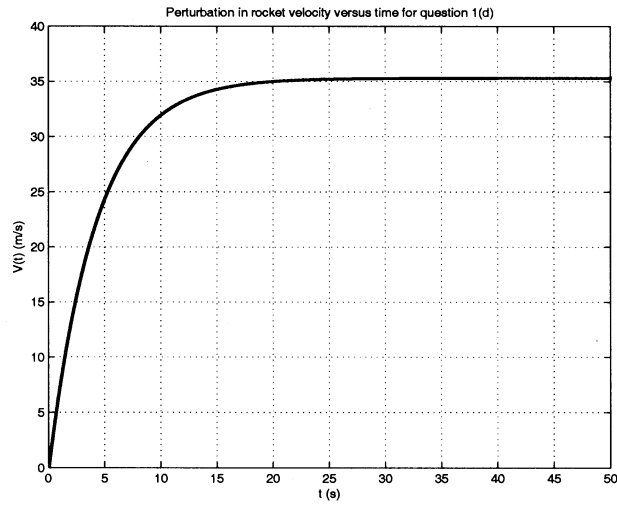
Figure 1: Velocity perturbation response of rocket with unit step input in thrust perturbation.
